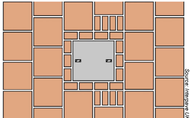
Figure 26. Using concrete pavers to fill around a utility cover
