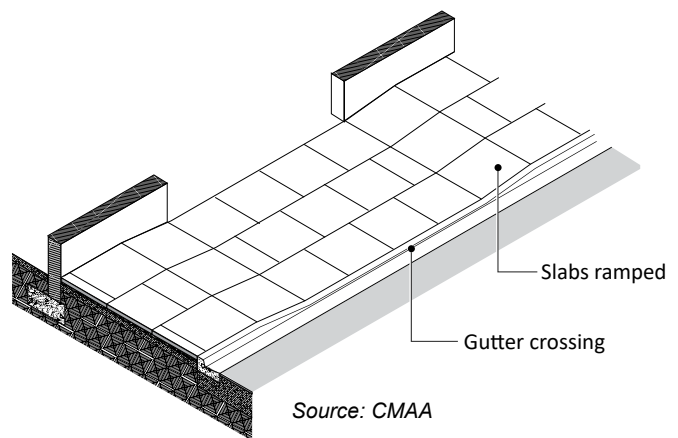
Figure 31. Driveway entrance with a depressed sidewalk surface.
